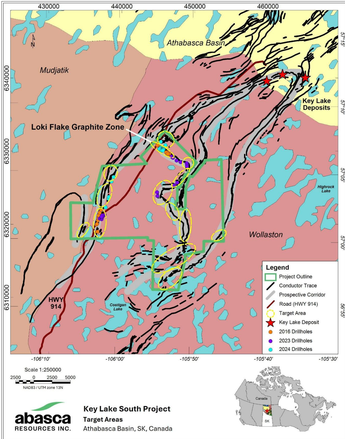
Figure 1: Map of the Key Lake South Project area showing the location of the Loki Flake Graphite Zone as well as several priority target areas for uranium exploration along prospective corridors.
